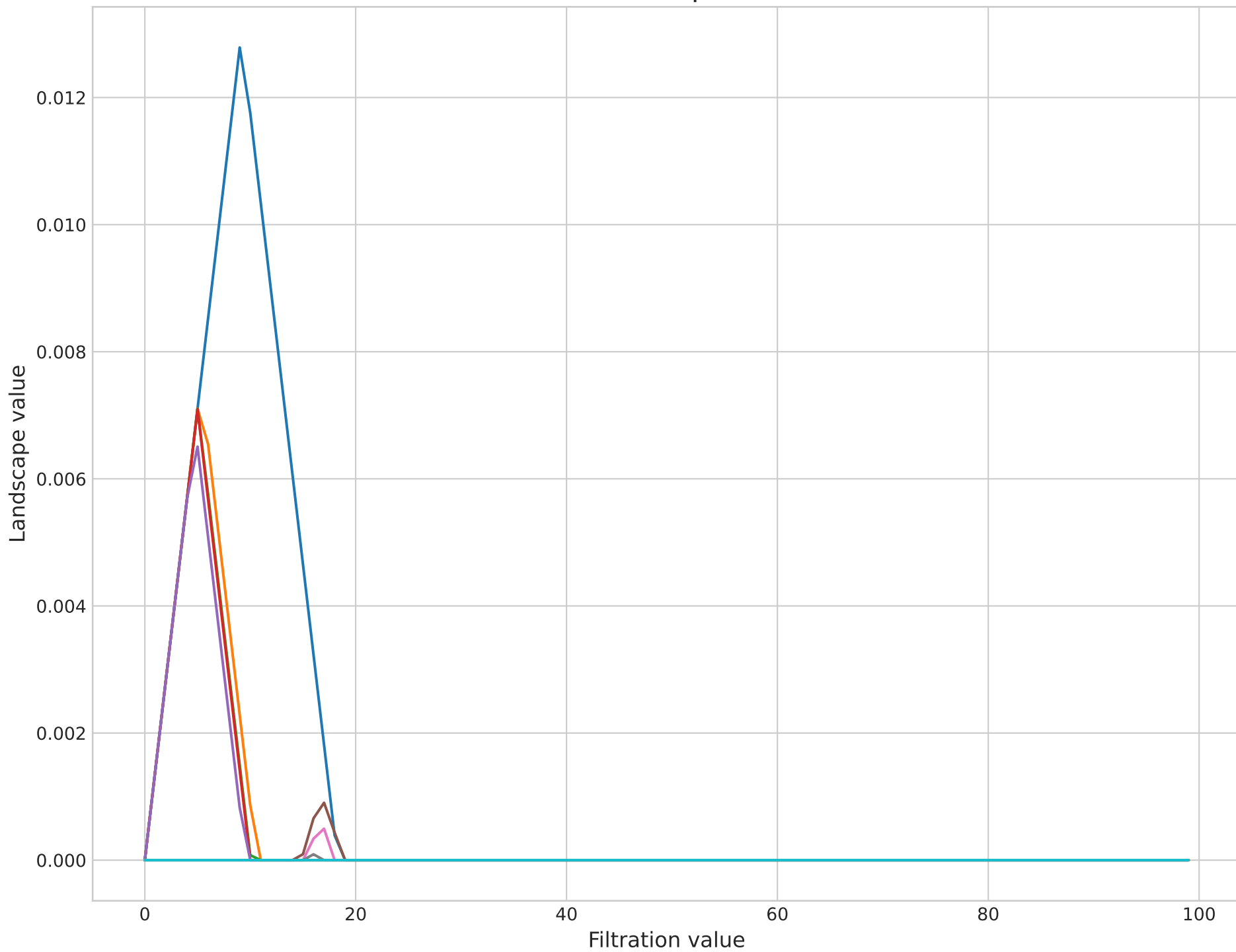
Persistence Landscape - Window 585
