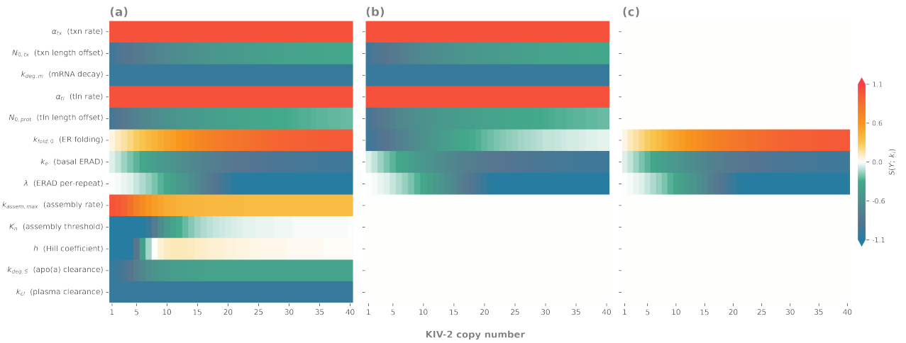
Figure 4: Normalized local sensitivity heatmaps. Sensitivity coefficients S(Y; k_i) for (a) plasma Lp(a) P_{ss} , (b) ER apo(a) load E_{ss} , and (c) ER secretion efficiency \eta_{ER} , evaluated at posterior median parameters. Warm colors indicate positive sensitivity; cool colors indicate negative sensitivity. KIV-2 copy number on the x-axis; model parameters on the y-axis.
