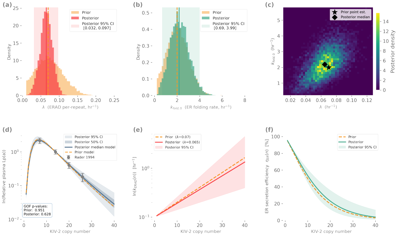
Figure 3: Bayesian prior-to-posterior for ERAD kinetics and model predictions. (a) Marginal distributions for \lambda (ERAD per-repeat susceptibility, \text{hr}^{-1} \text{ repeat}^{-1} ); dashed vertical line indicates prior point estimate; solid vertical line indicates posterior median; shaded band shows posterior 95% credible interval. (b) Marginal distributions for k_{fold,0} (ER folding rate constant, \text{hr}^{-1} ); same conventions as (a). (c) Joint 2D posterior density for (\lambda, k_{fold,0}) ; star indicates prior point estimate; diamond indicates posterior median. (d) Normalized plasma Lp(a) P_{ss}(n)/P_{ss}(14) versus KIV-2 copy number; dashed line shows prior model; solid line shows posterior median model; shaded bands show posterior 50% and 95% credible envelopes; gray points show Rader 1994 production rate data ( \pm SEM). (e) ERAD rate k_{ERAD}(n) = k_e \cdot e^{\lambda n} on a log scale; dashed line shows prior, solid line shows posterior median, shaded band shows posterior 95% credible interval propagated across 500 posterior draws. (f) ER secretion efficiency \eta_{ER}(n) [%]; same conventions as (e). All posterior results are based on 4 chains \times 2000 NUTS draws ( \hat{R} < 1.01 ), conditioned on isoform-specific production rate data from Rader et al. 14 at n = 7, 14, 20, 26 .
