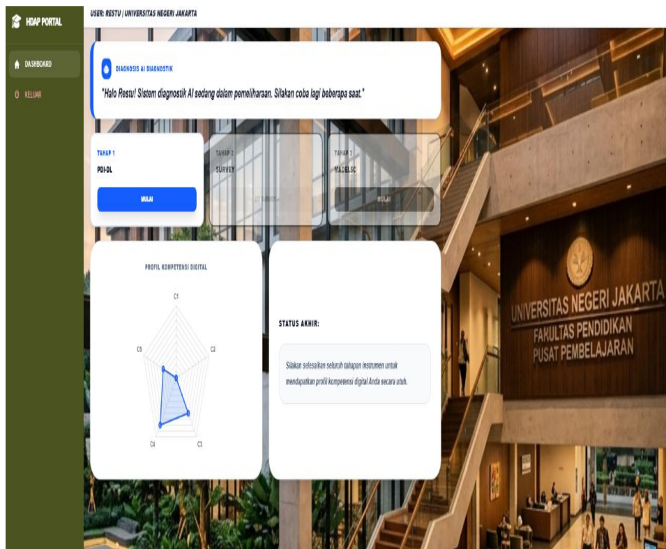
Gambar 3 Dashboard USER
