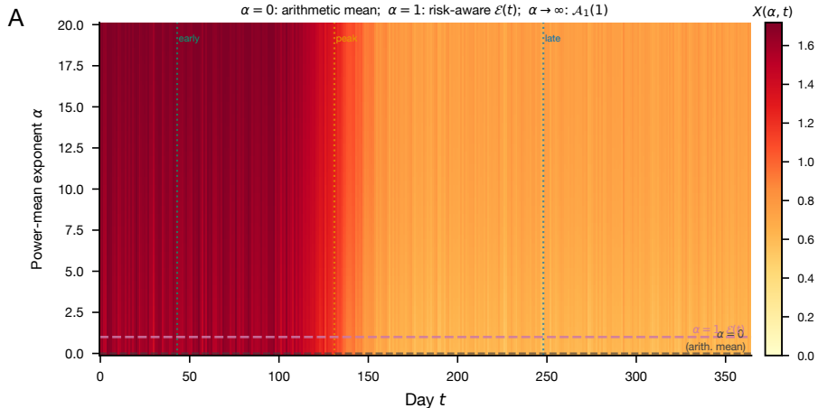
Power-mean reproduction-number spectrum X(\alpha, t) — Scenario_A
