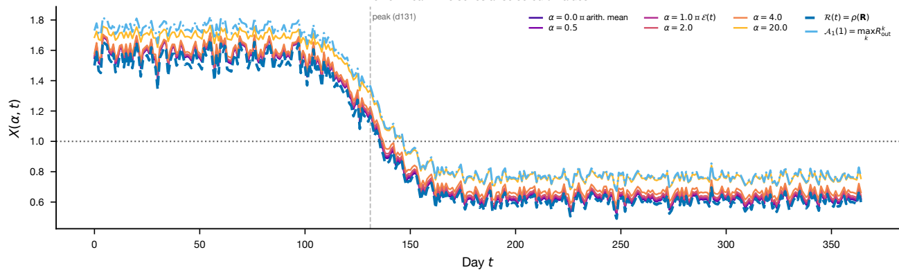
Power-mean time series at selected \alpha values
