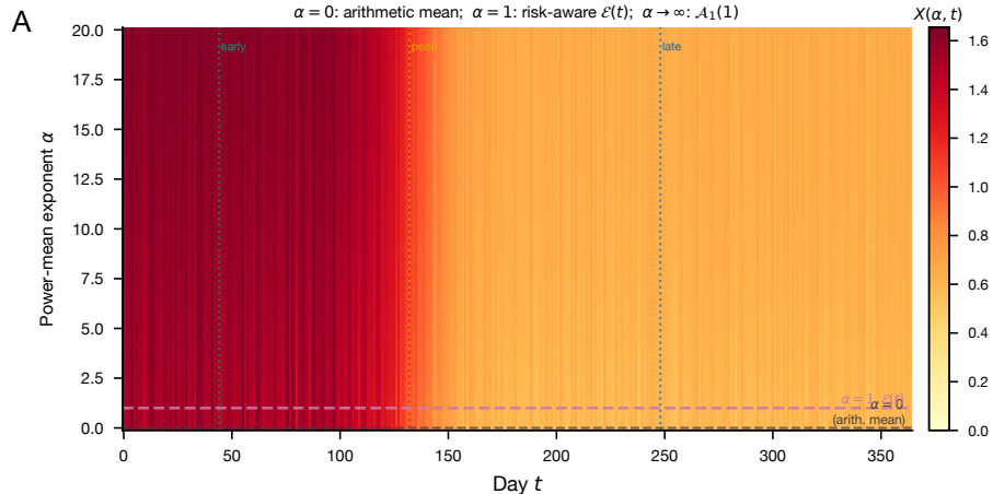
Power-mean reproduction-number spectrum X(\alpha, t) — Scenario_C
