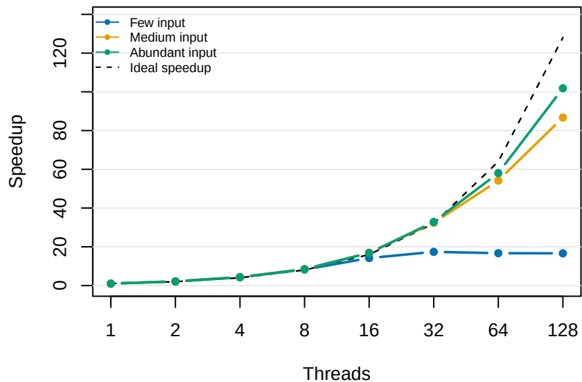
Across-wires: total speedup
