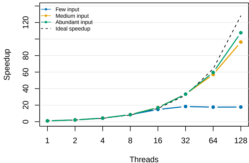
Across-wires: computation speedup
