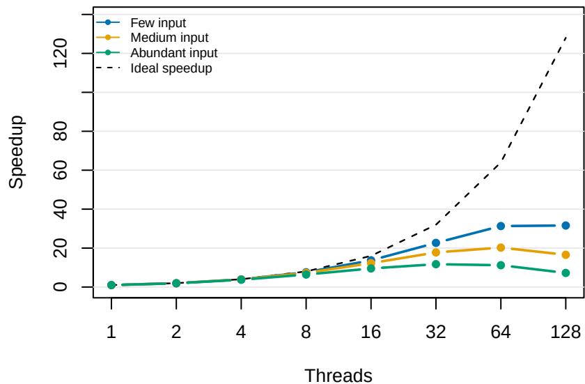
Within-wires: total speedup
