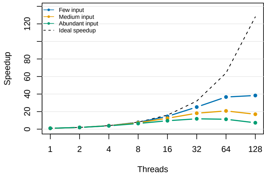
Within-wires: computation speedup
