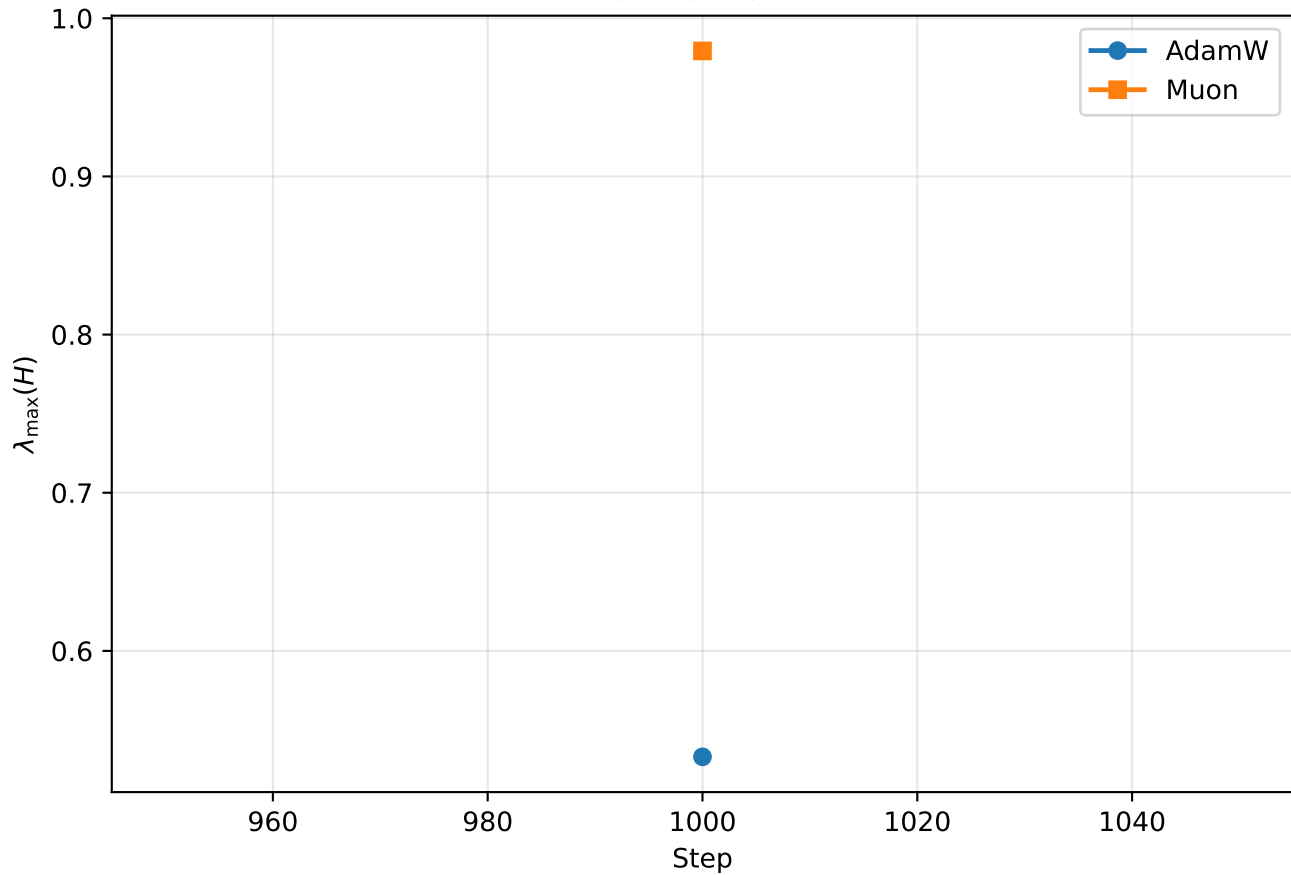
Chinchilla-1
