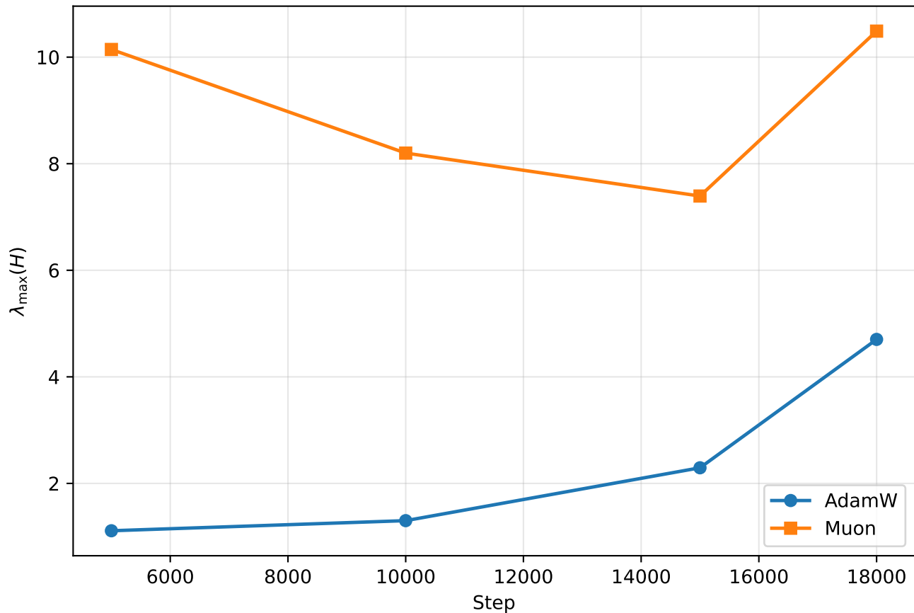
Chinchilla-16
