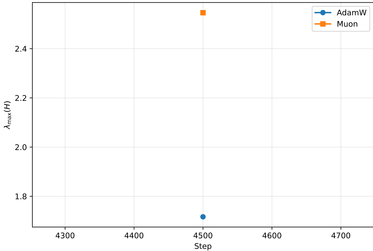
Chinchilla-4
