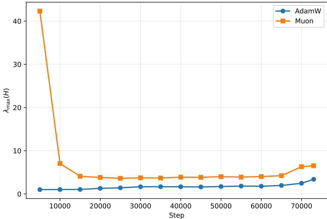
Chinchilla-64
