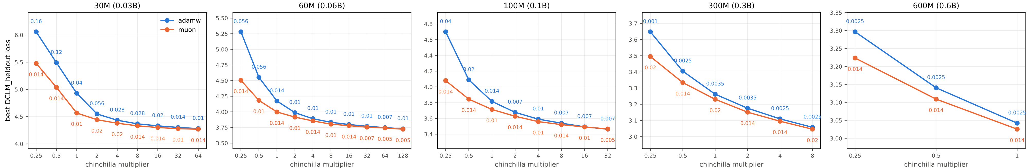
Best-LR held-out DCLM loss vs token budget (wd 0.1, batch 1M)
