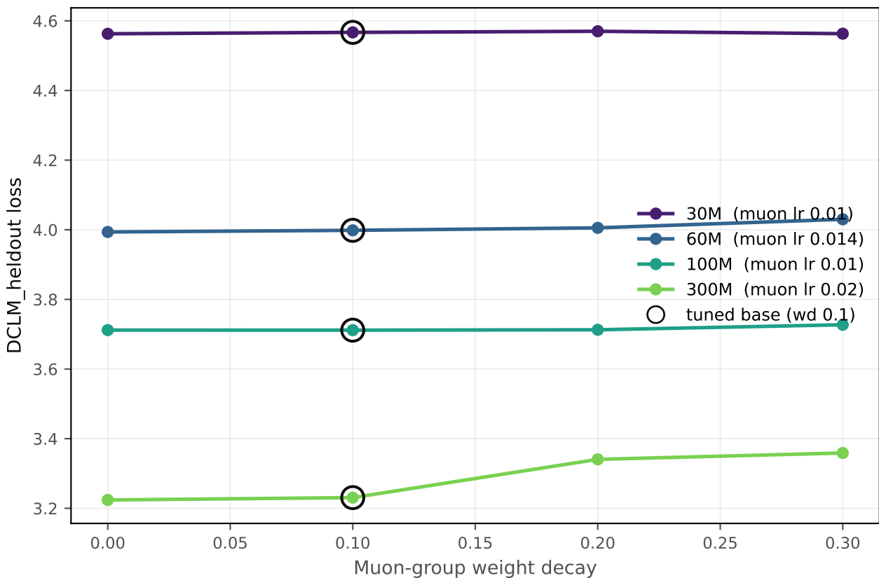
Held-out DCLM loss vs Muon weight decay at chinchilla 1 — AdamW group held at wd 0.1
