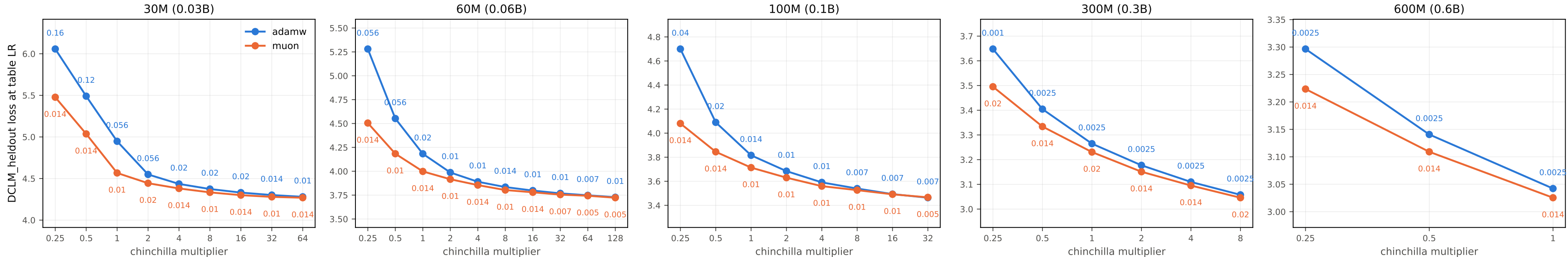
Held-out DCLM loss at the PT_LR_BY_MODEL table's LRs (wd 0.1, batch 1M)
