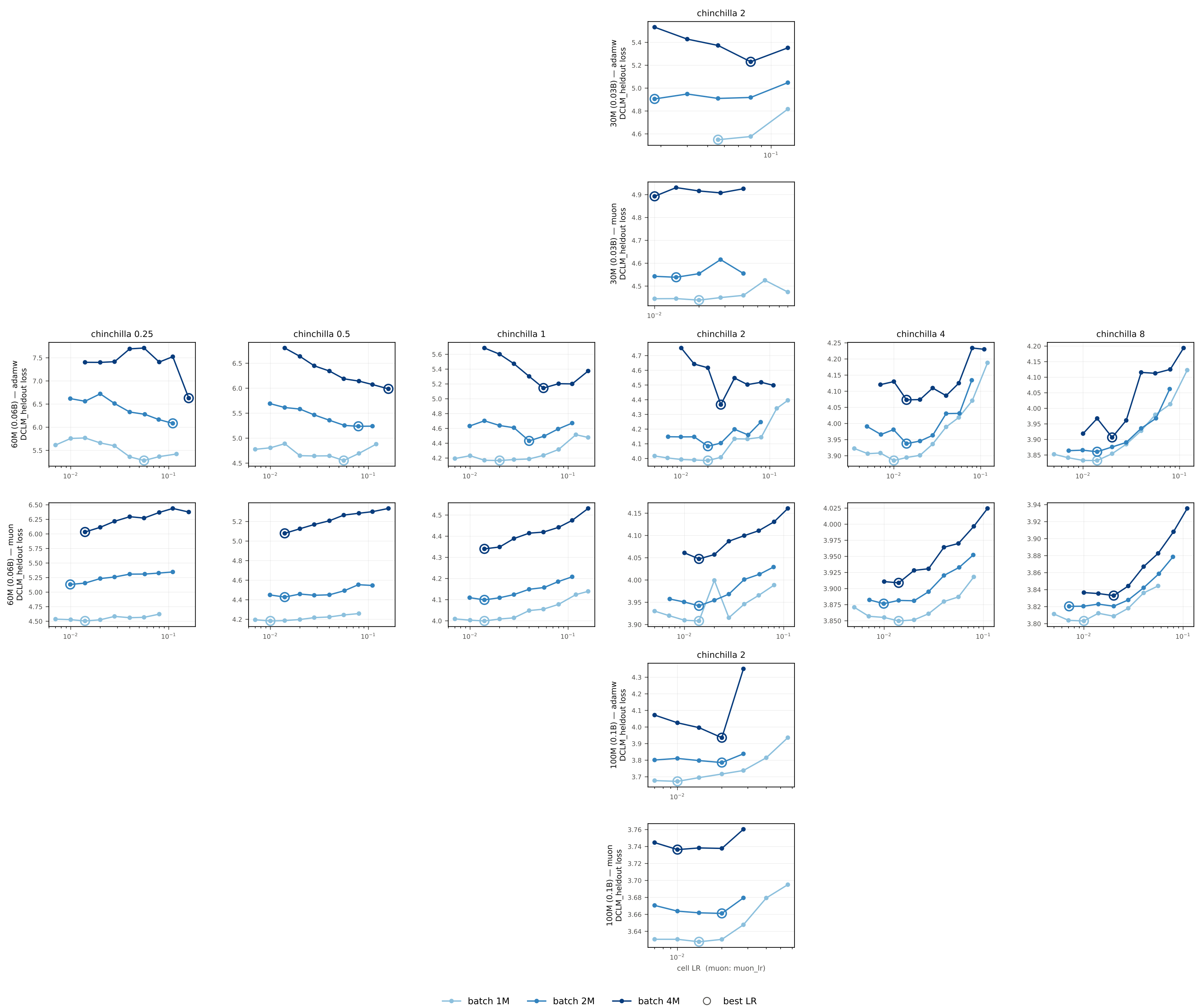
Pretrain LR vs held-out DCLM loss across global batch size, every size x token budget (wd 0.1) — 4,193,280 eval tokens/point
