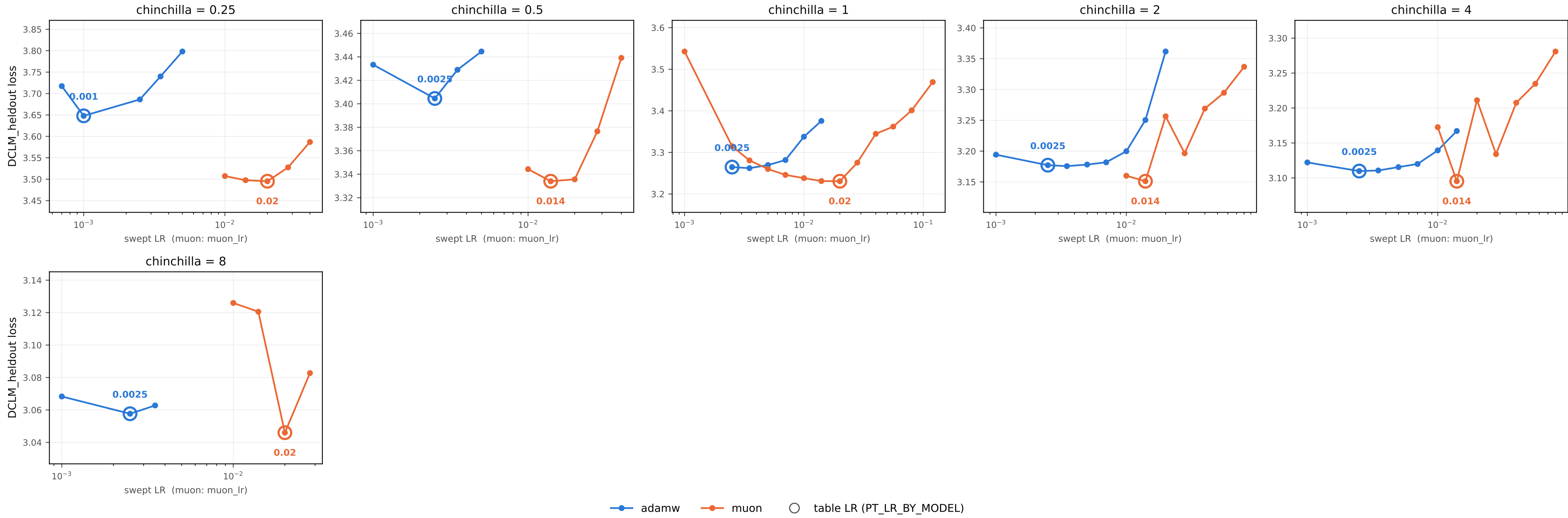
300M (0.3B), wd 0.1 / batch 1M: pretrain LR vs held-out DCLM loss — 4,193,280 eval tokens per point
