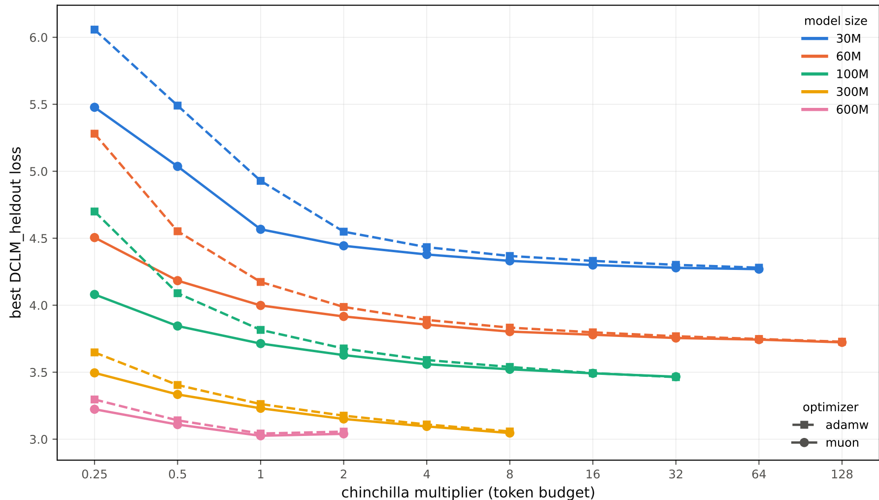
Best-LR held-out DCLM loss vs token budget, all model sizes (wd 0.1, batch 1M)
