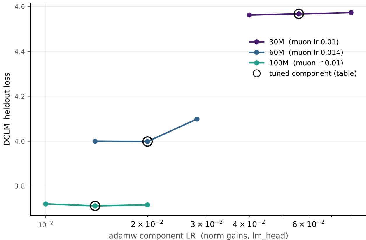
Held-out DCLM loss vs adamw component at chinchilla 1 — muon lr fixed at the tuned value, wd 0.1
