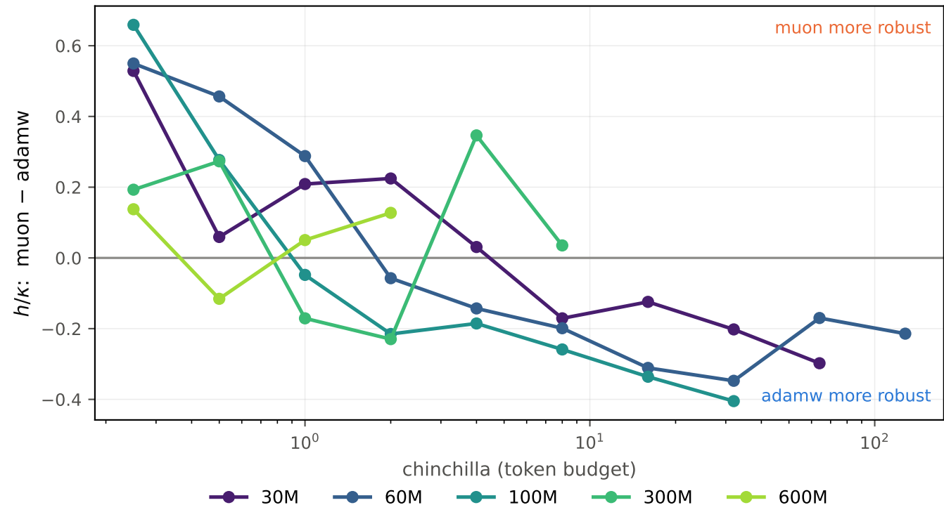
Crossover in h/k with token budget
