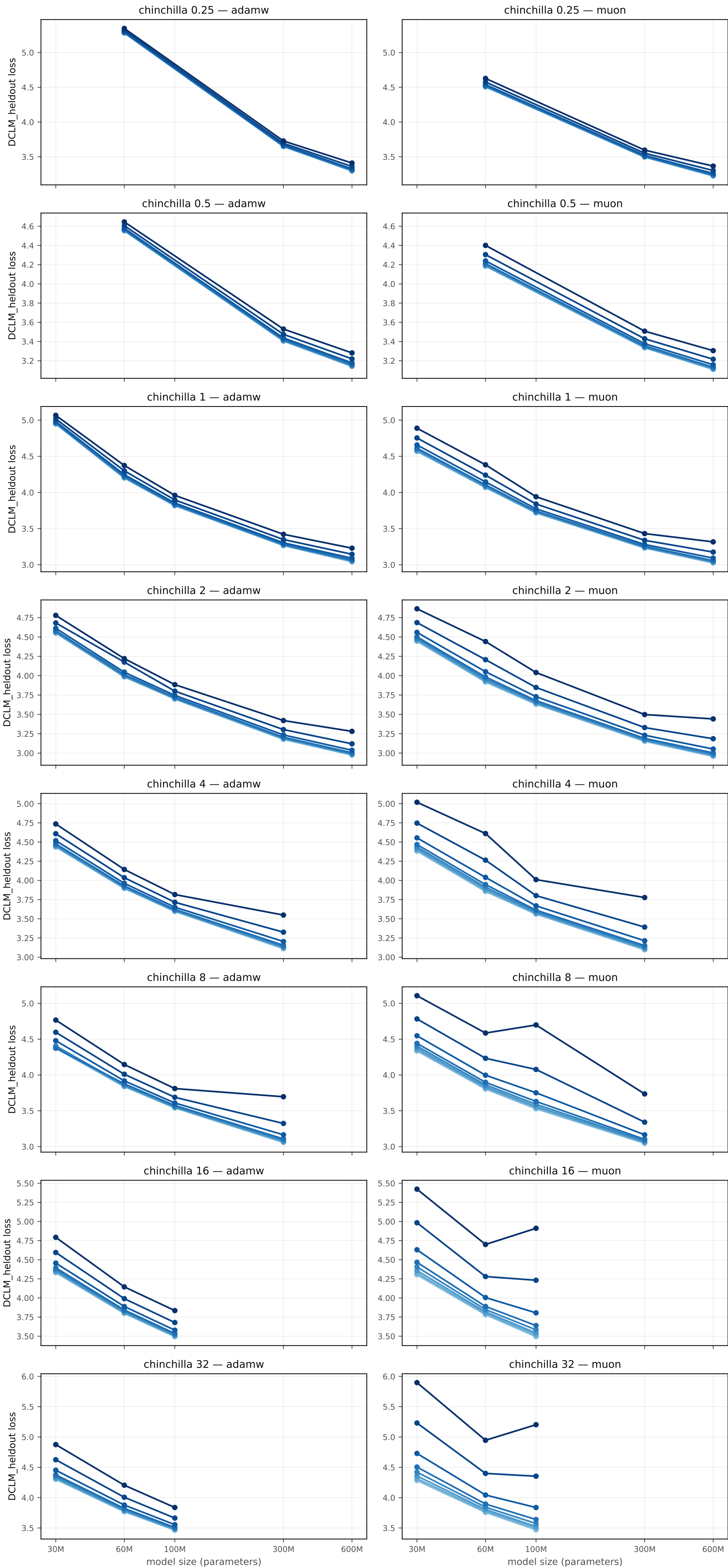
Post-perturbation held-out DCLM loss, by model size
