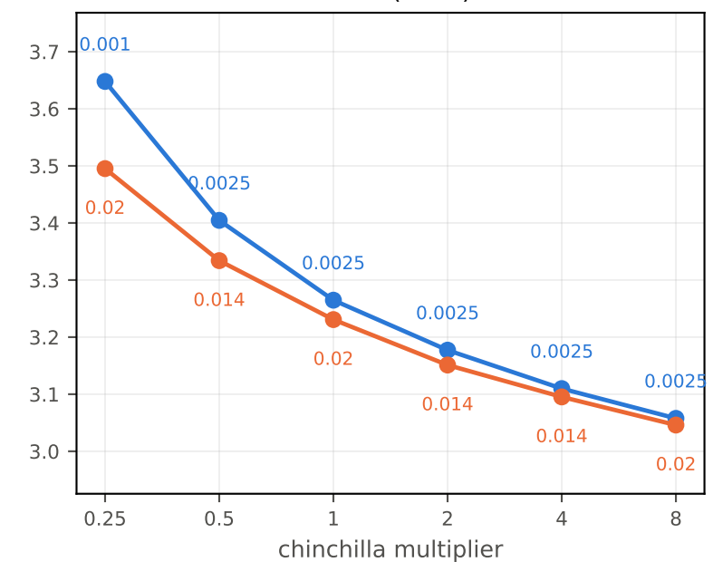
300M (0.3B)
