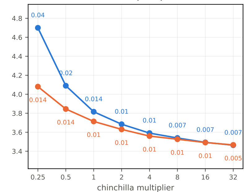
100M (0.1B)
