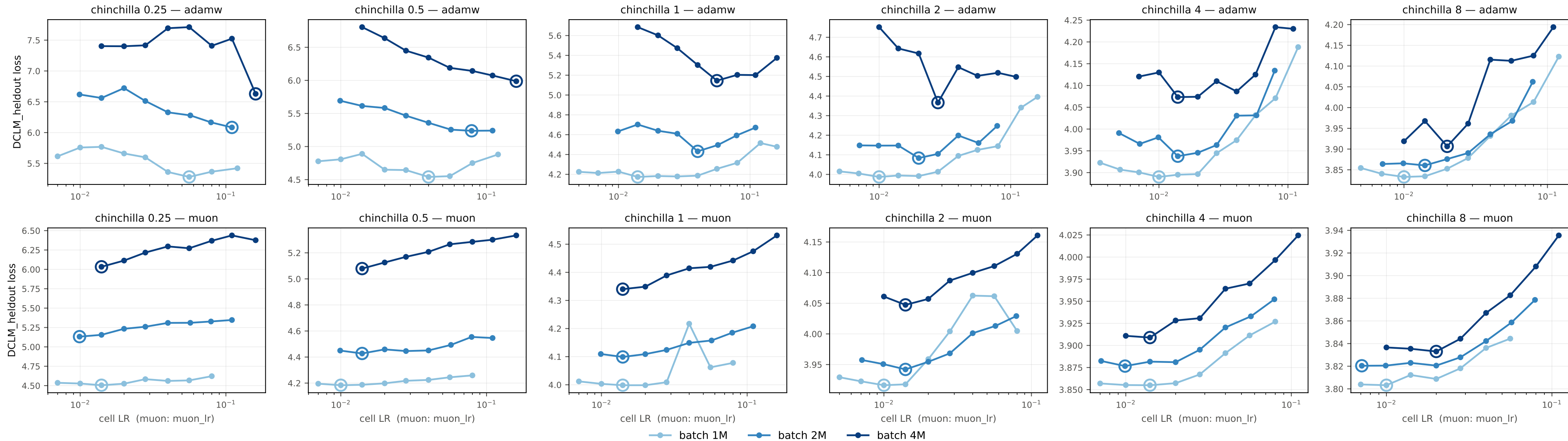
60M (0.06B), wd 0.1: pretrain LR vs held-out DCLM loss across global batch size — 4,193,280 eval tokens/point
