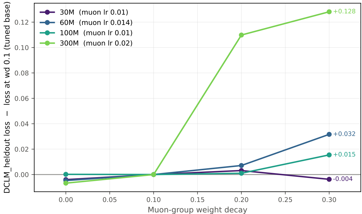
Muon weight decay at chinchilla 1, AdamW group held at wd 0.1 — change in held-out DCLM loss vs the tuned base
