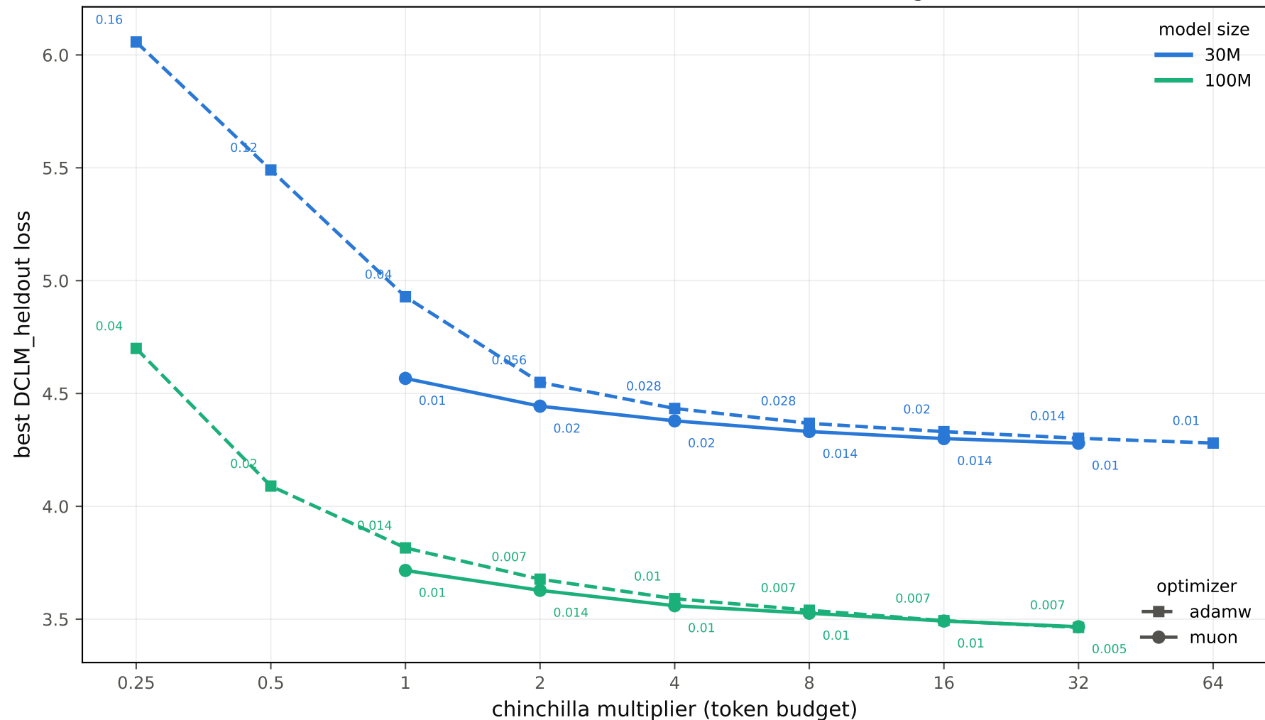
Best-LR held-out DCLM loss vs token budget, all model sizes (wd 0.1, batch 1M; annotation = the winning LR)
