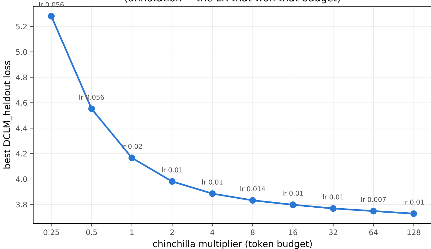
60M adamw: loss of the best-LR model vs token budget (annotation = the LR that won that budget)
