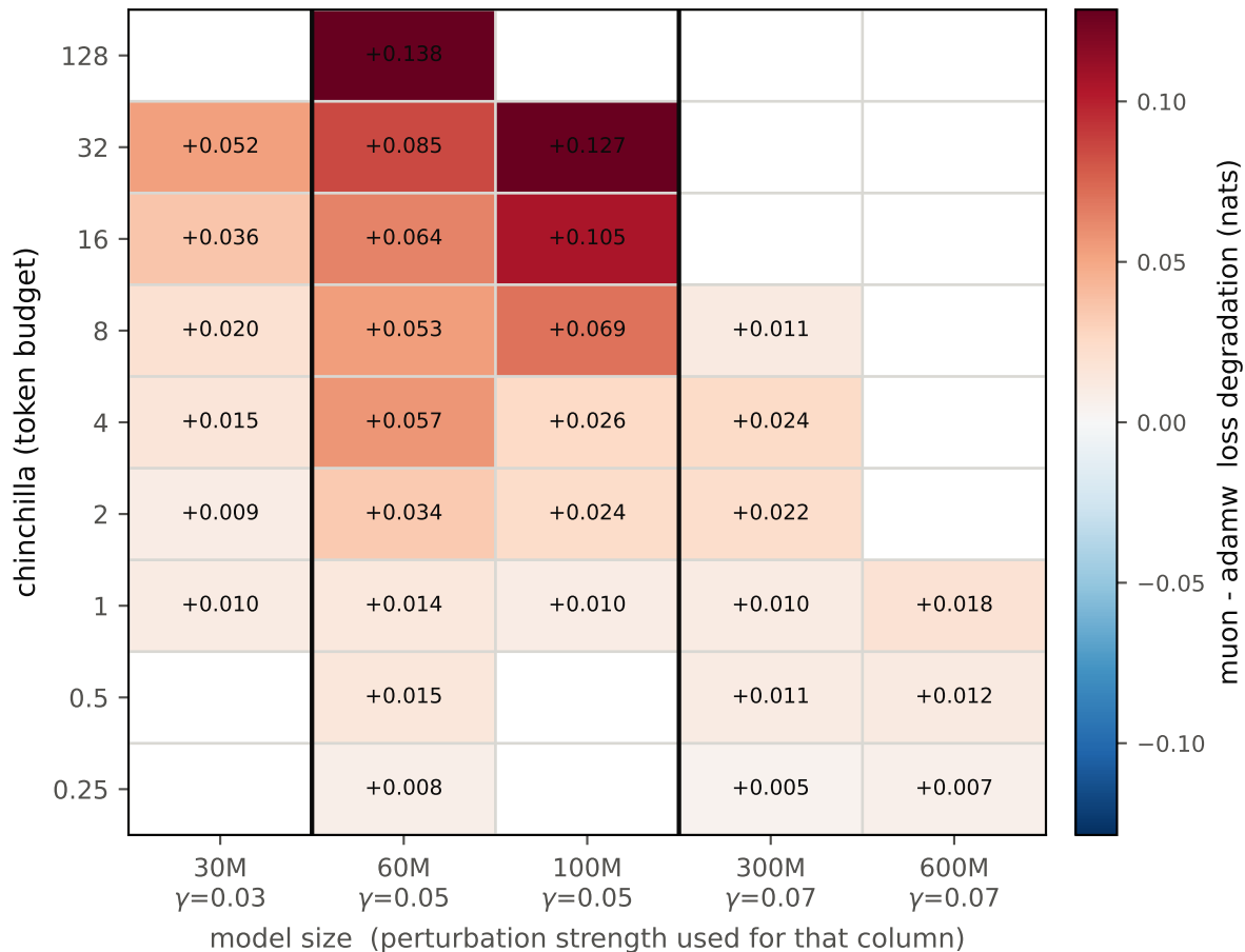
Degradation under Gaussian weight perturbation: muon vs adamw size-matched \gamma per column
