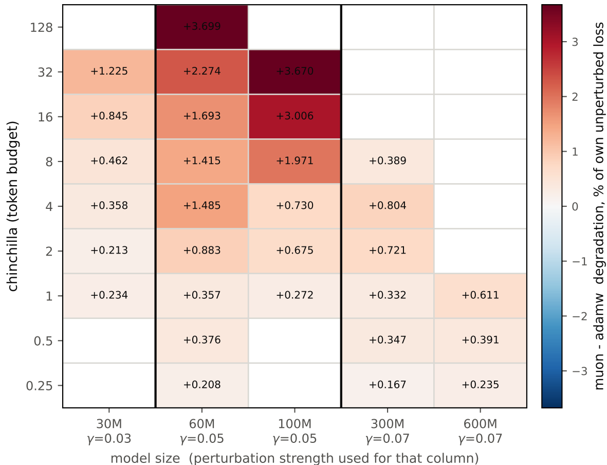
Relative degradation under Gaussian weight perturbation: muon vs adamw size-matched \gamma per column
