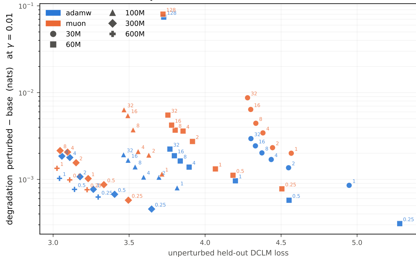
Degradation under Gaussian weight perturbation ( \gamma = 0.01 ) vs model quality every tuned base; small label = chinchilla
