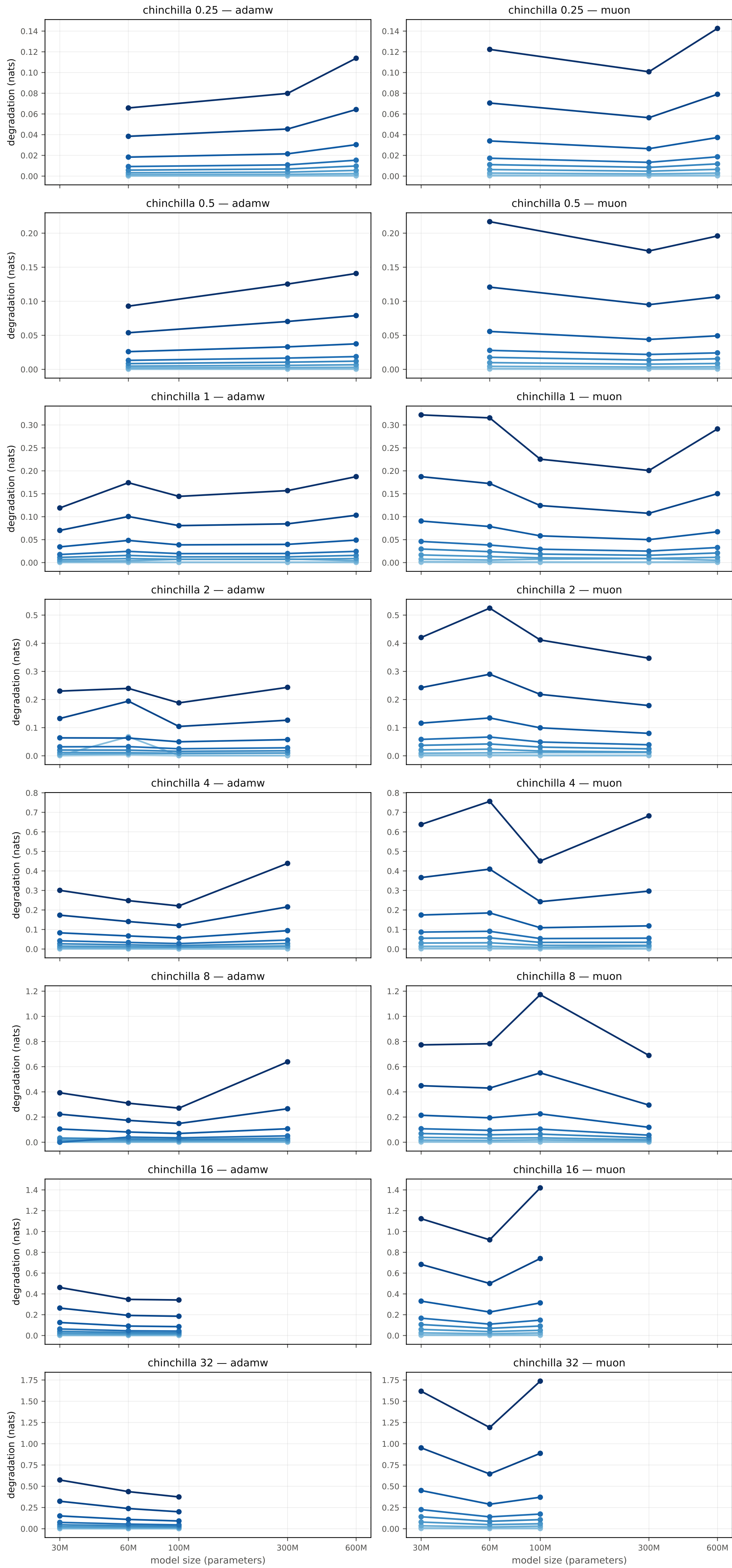
Loss degradation from Gaussian weight perturbation (perturbed - unperturbed), by model size
