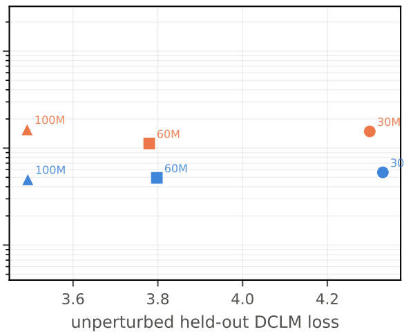
chinchilla 16
