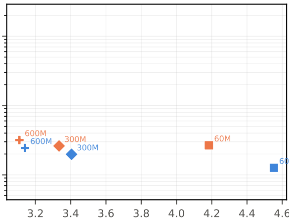
chinchilla 16
