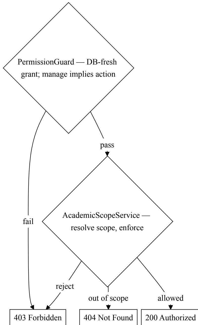
Figure 7.5. Authorization decision chain for a tenant-scoped request, part 2: permission evaluation and academic-scope enforcement outcomes.
