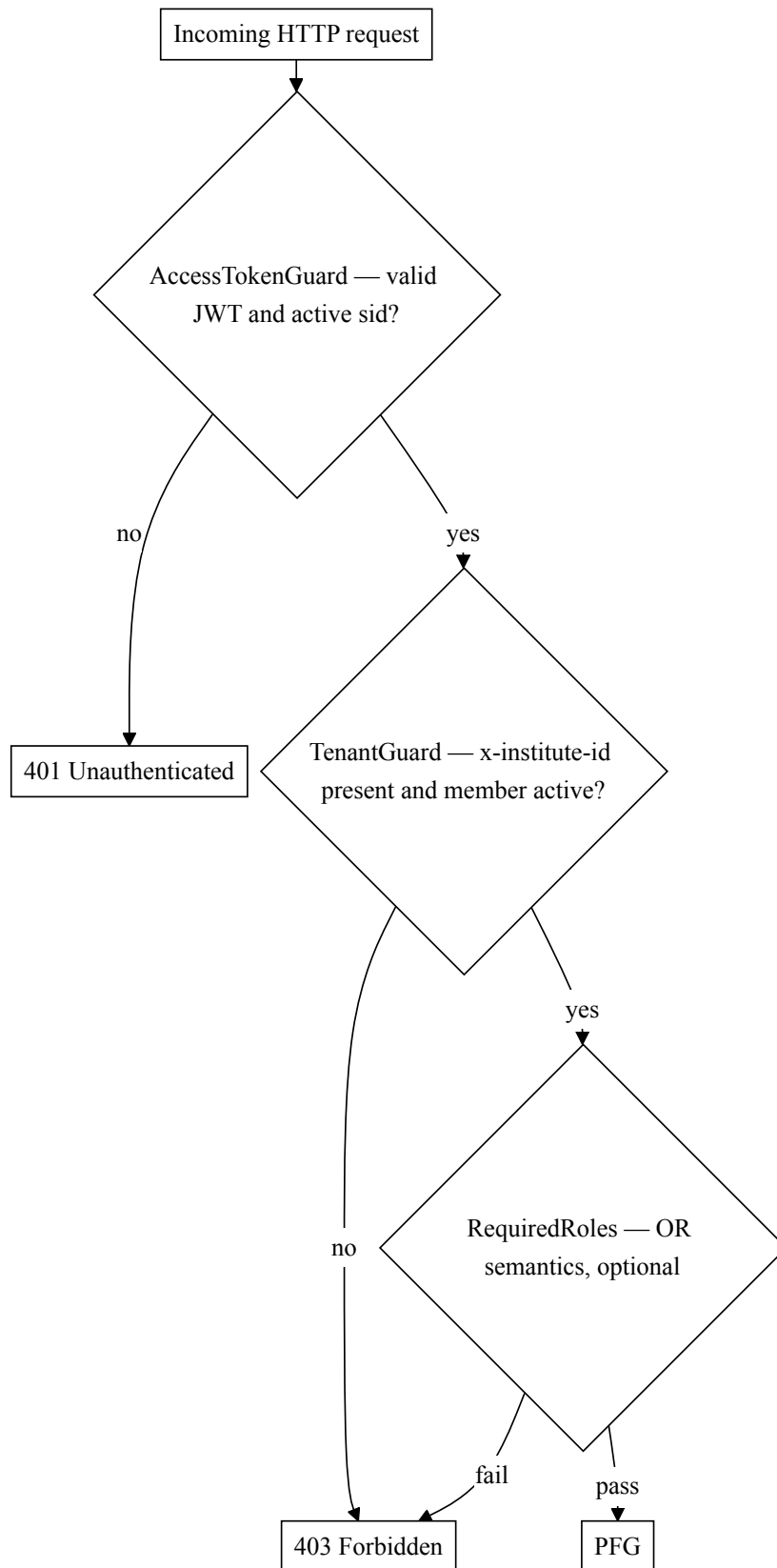
Figure 7.4. Authorization decision chain for a tenant-scoped request, part 1: the guard-stage decisions.
