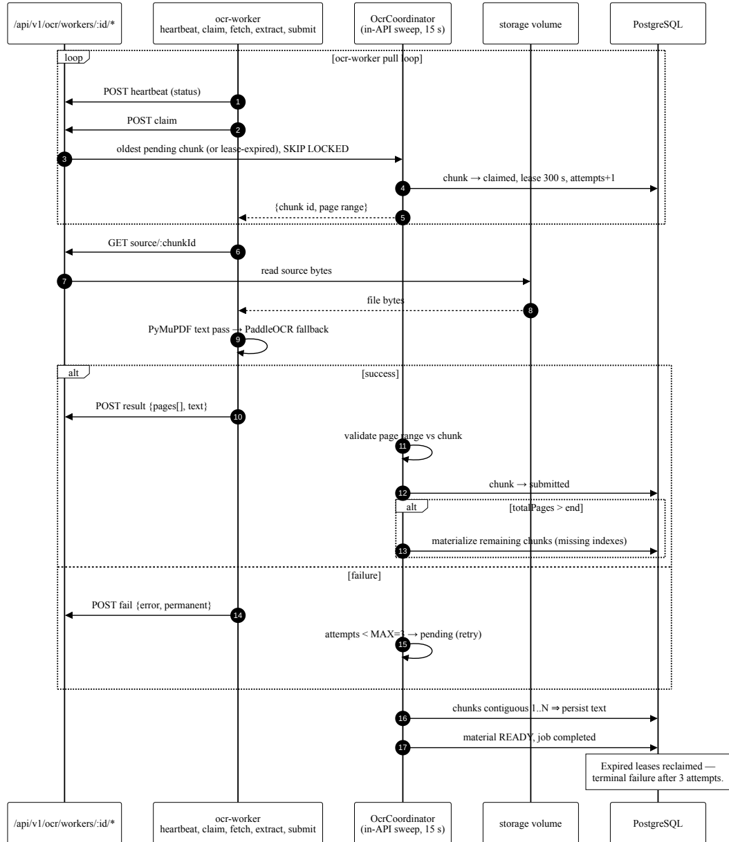
Figure 8.2. Distributed OCR material processing, part 2: worker pull, extraction, and settlement.
