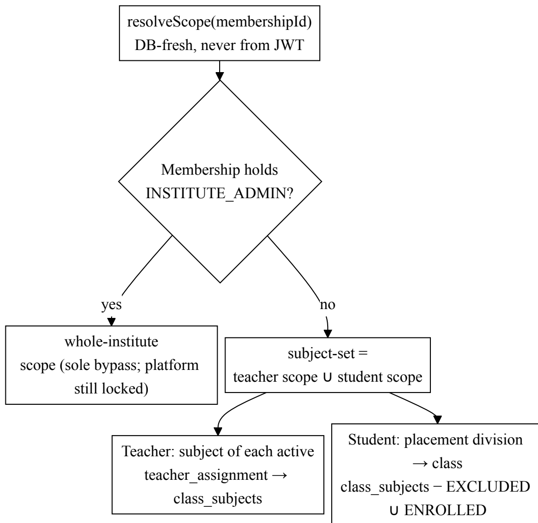
Figure 7.6. Academic scope — resolution of the actor's subject set from database state.
