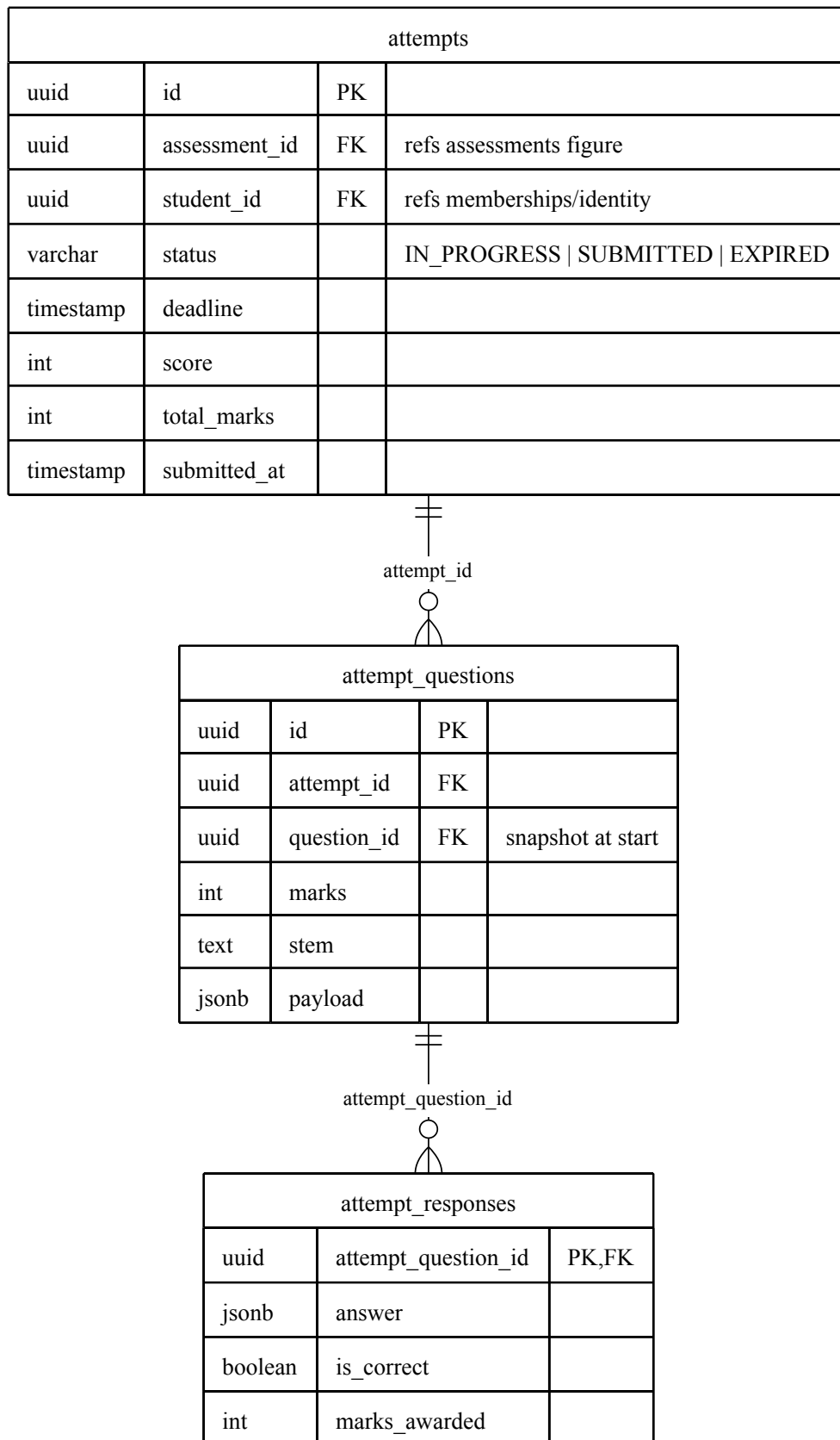
Figure 6.12. Database schema — attempt snapshots and response tables.
