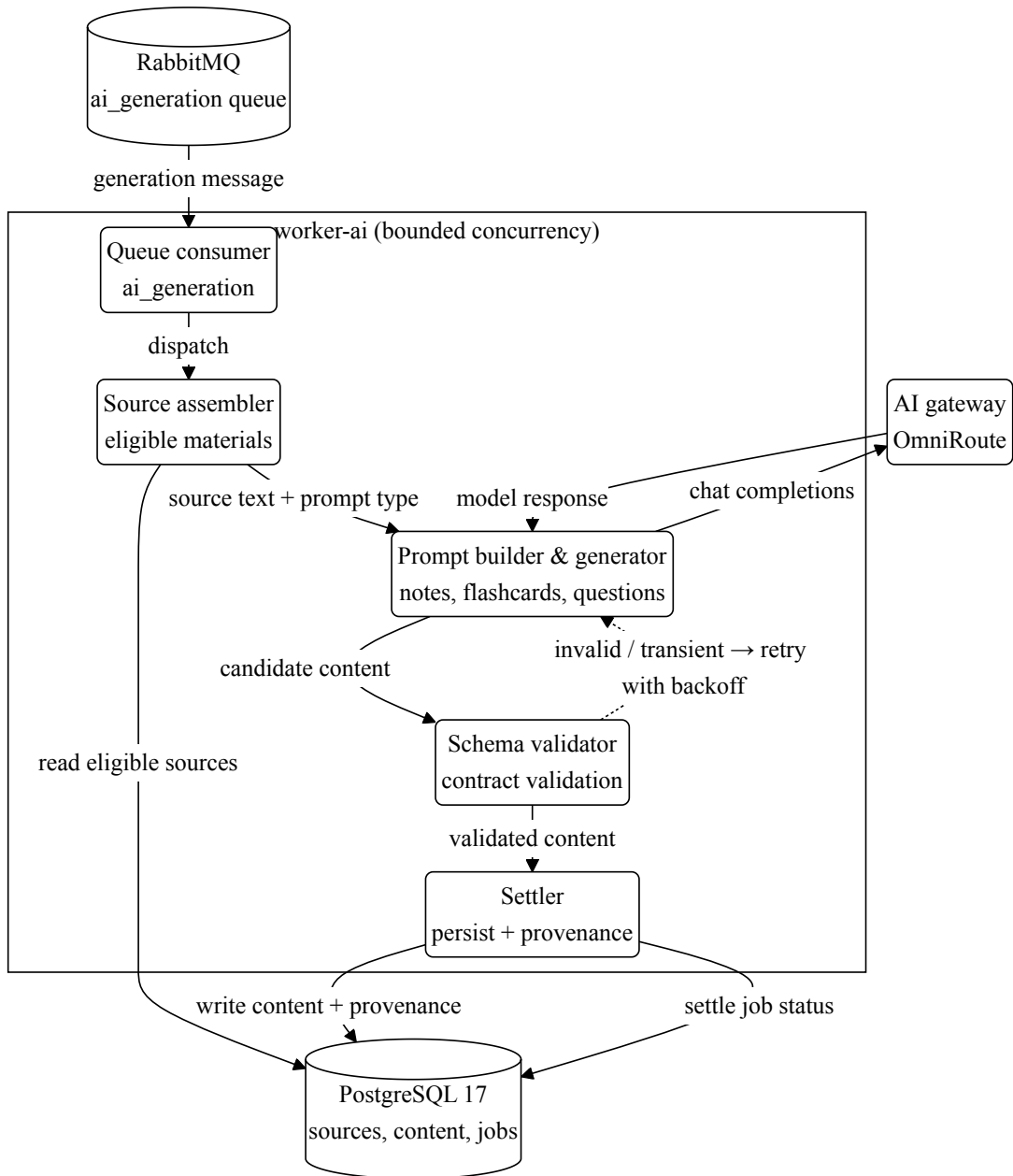
Figure 5.6. Level-3 data flow diagram: the AI generation pipeline inside worker-ai .
