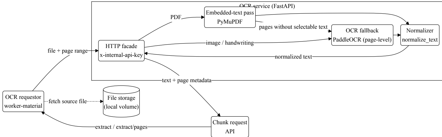
CatLium EduTech — Level-2 DFD (b): OCR service extraction pipeline
