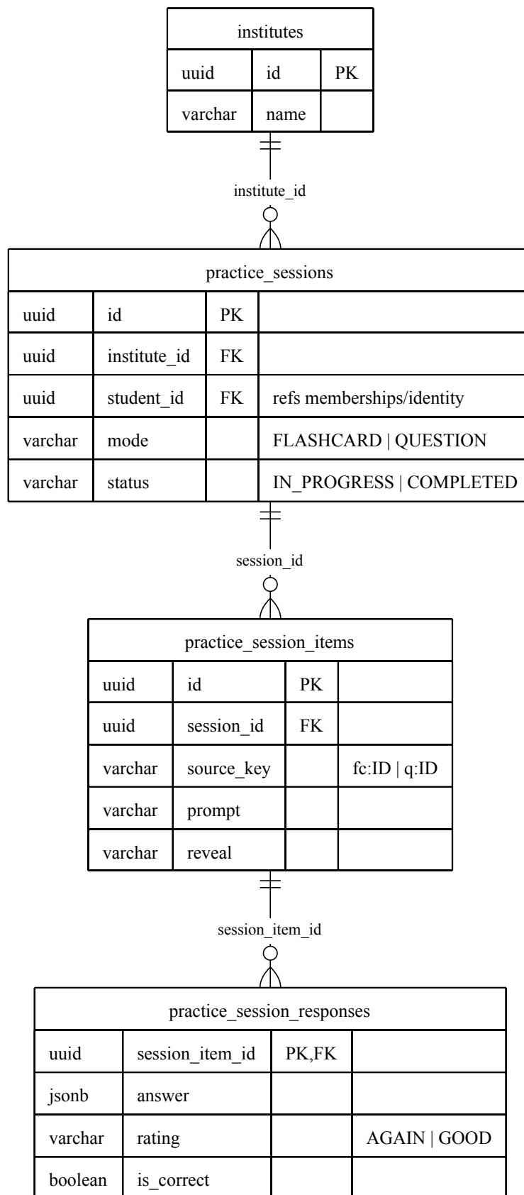
Figure 3.13. Database schema — ungraded practice sessions.
