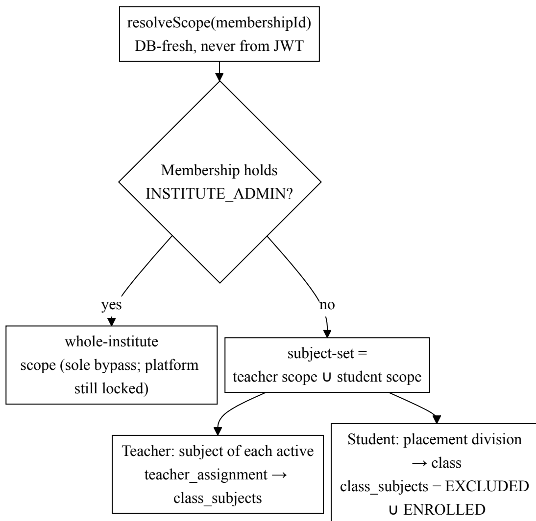
Figure 4.6. Academic scope — resolution of the actor's subject set from database state.
