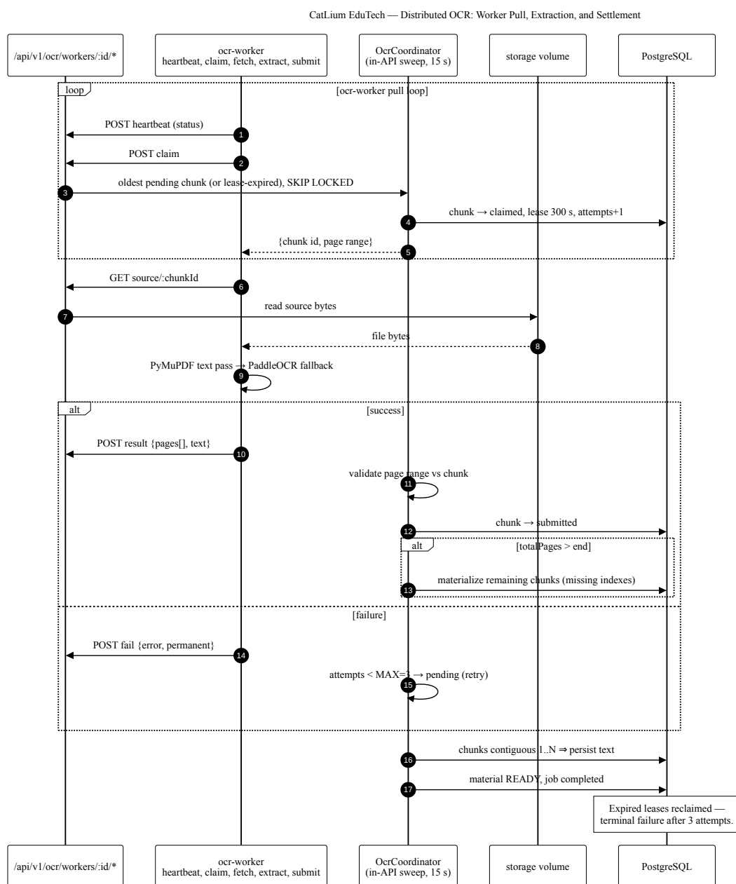
Figure 5.2. Distributed OCR material processing, part 2: worker pull, extraction, and settlement.
