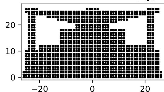
Free-form: Side view (z,y)
