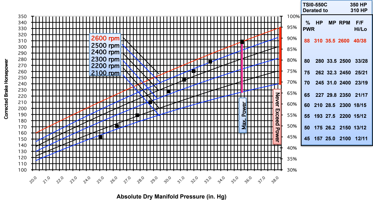
Sea Level Constant Speed Curve ( TSI0-550-C )
