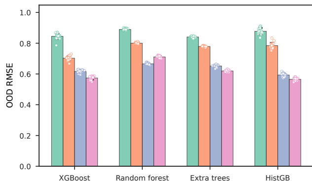
(c) OOD RMSE by descriptor layer
