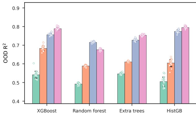
(a) OOD R 2 by descriptor layer
