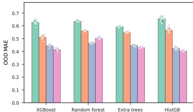
(b) OOD MAE by descriptor layer
