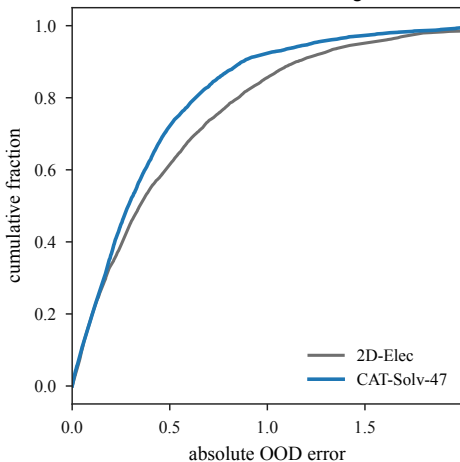
Distribution-level error migration
