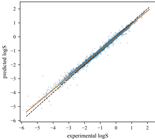
GNN + \sigma IID parity
