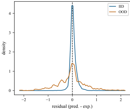
GNN residual concentration
