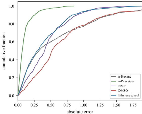
GNN OOD error by solvent
