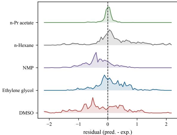
GNN residual ridges by solvent
