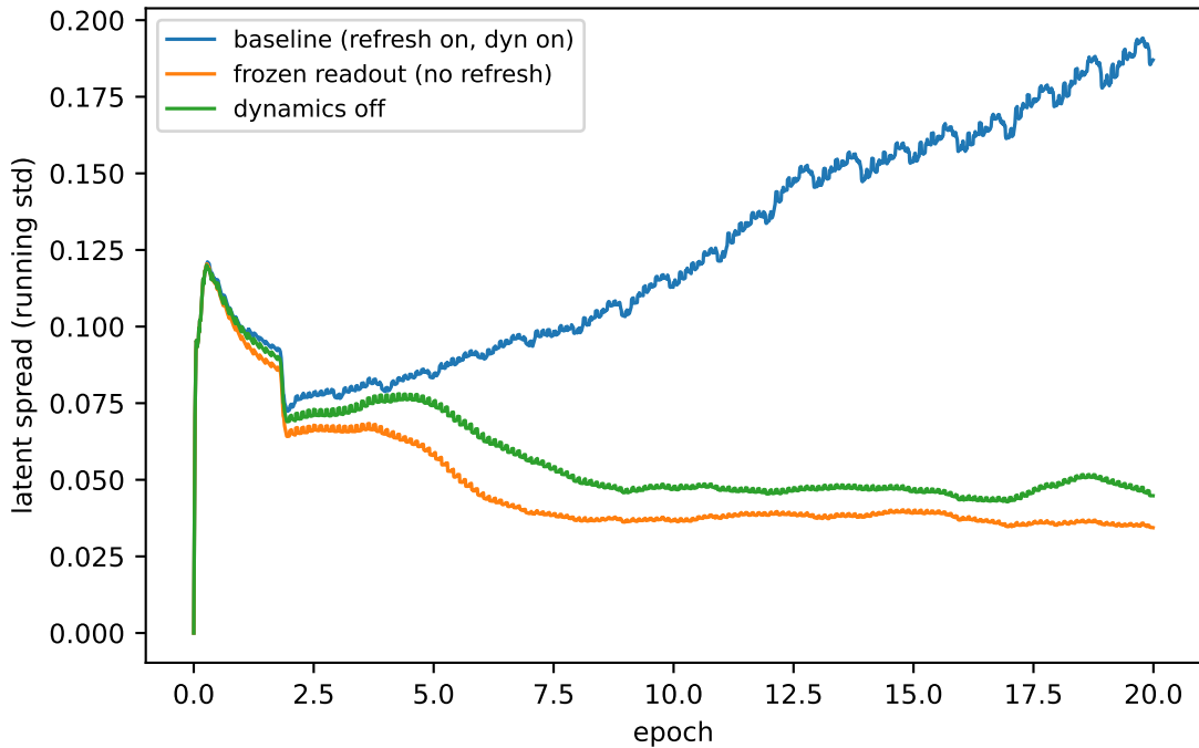
What drives the latent inflation? (dir 225 deg, L=2, 20 ep)
