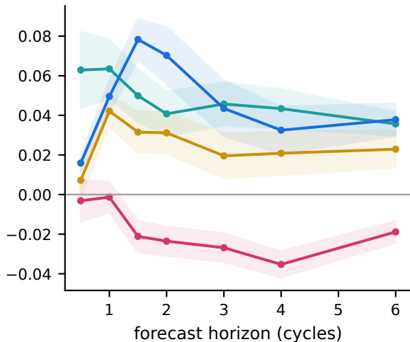
vs PSTH (near-oracle)
