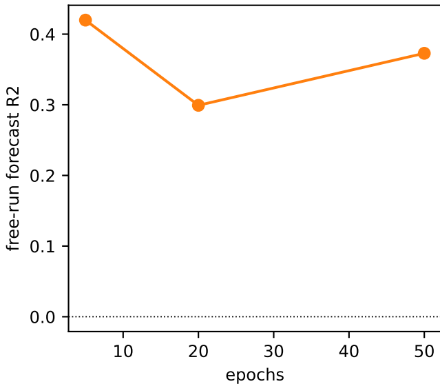
Single-direction sVJF (dir 225 deg, L=2): metrics vs epochs
