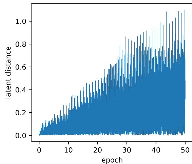
Dist: filtered latent > nearest RBF center
