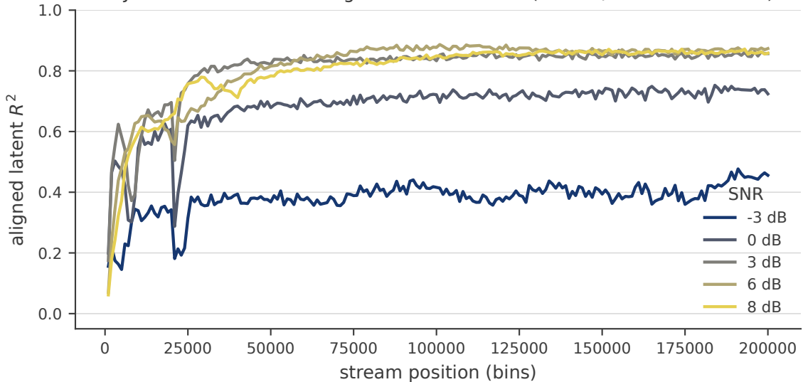
sVJF online readout converges over the stream (slower / lower at low SNR)
