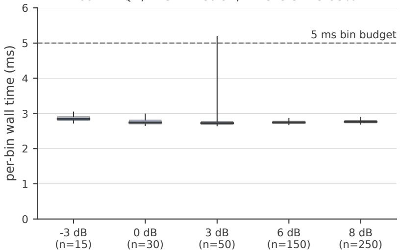
sVJF real-time per-bin latency (single core, Intel Xeon @ 2.20 GHz) box = IQR, line = median, whiskers = 5-95%
