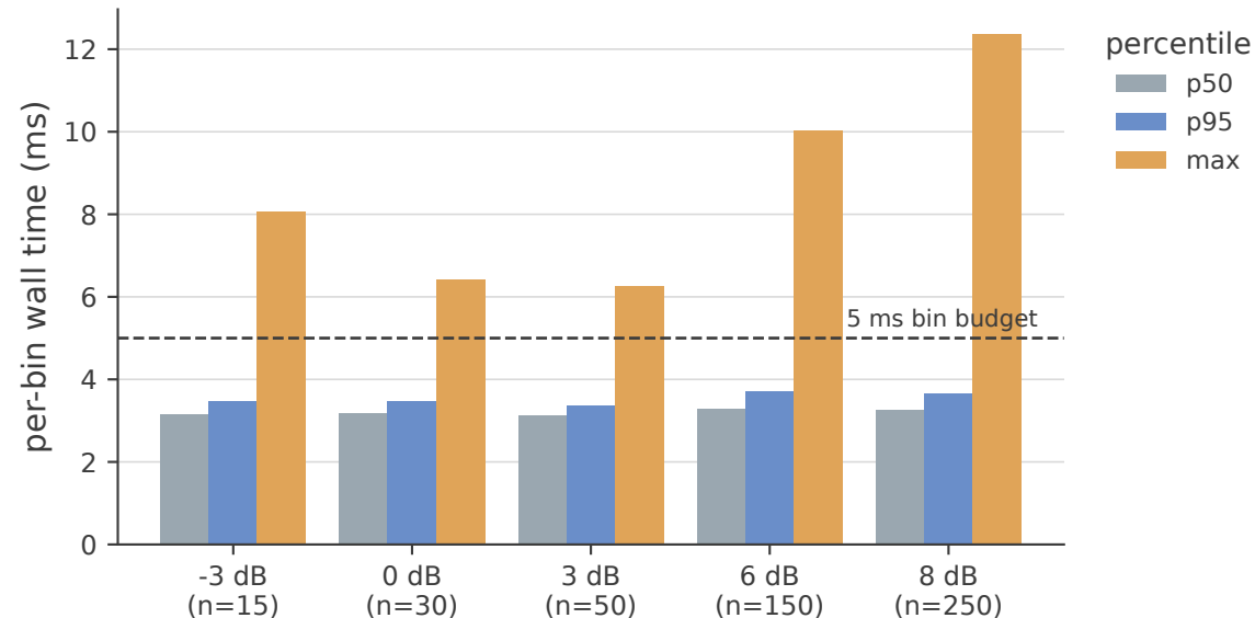
Real-time per-bin cost (online readout, e2-standard-4)
