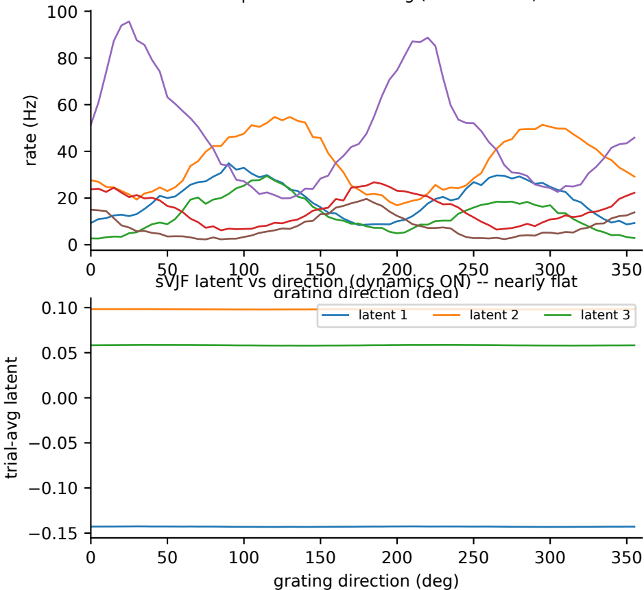
Example V1 neuron tuning (6 best-tuned)
