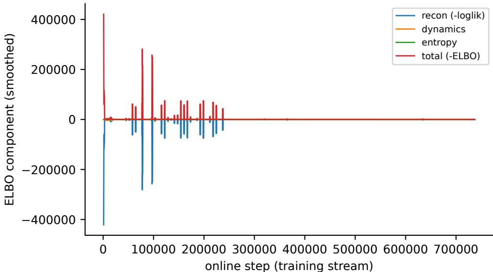
Training convergence over the single online pass
