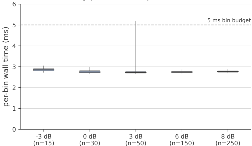
Real-time per-bin latency (single core, e2-standard-4) box = IQR, line = median, whiskers = 5-95%
